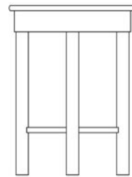
W-277-MO-R Round Night Table with shelf 18 DIA x 24H
