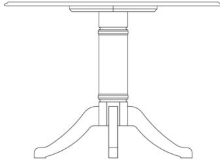
A-080-MO-4-DL Drop-Leaf Dining Table 42 DIA x 30H
