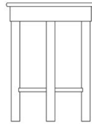
A-277-MO-R Round Night Table with shelf 18 DIA x 24H
